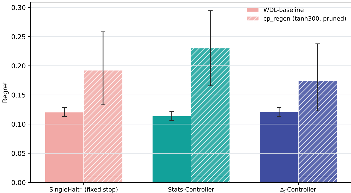
cp_regen (real regeneration under \tanh(\text{cp\_order}/300) + pruning) vs. WDL-baseline
