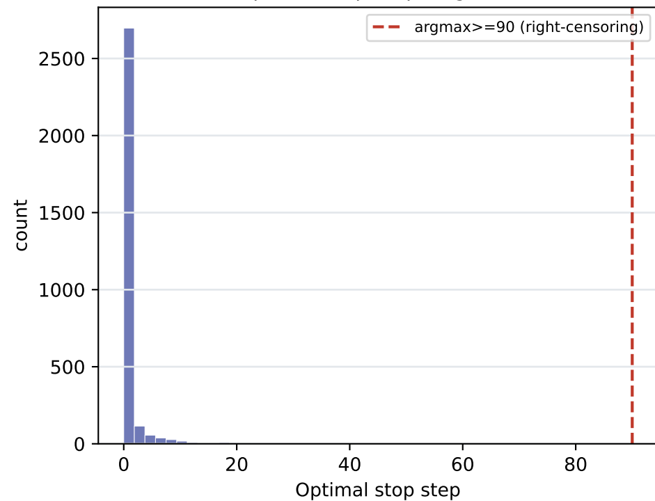
Optimal stop step (argmax)
