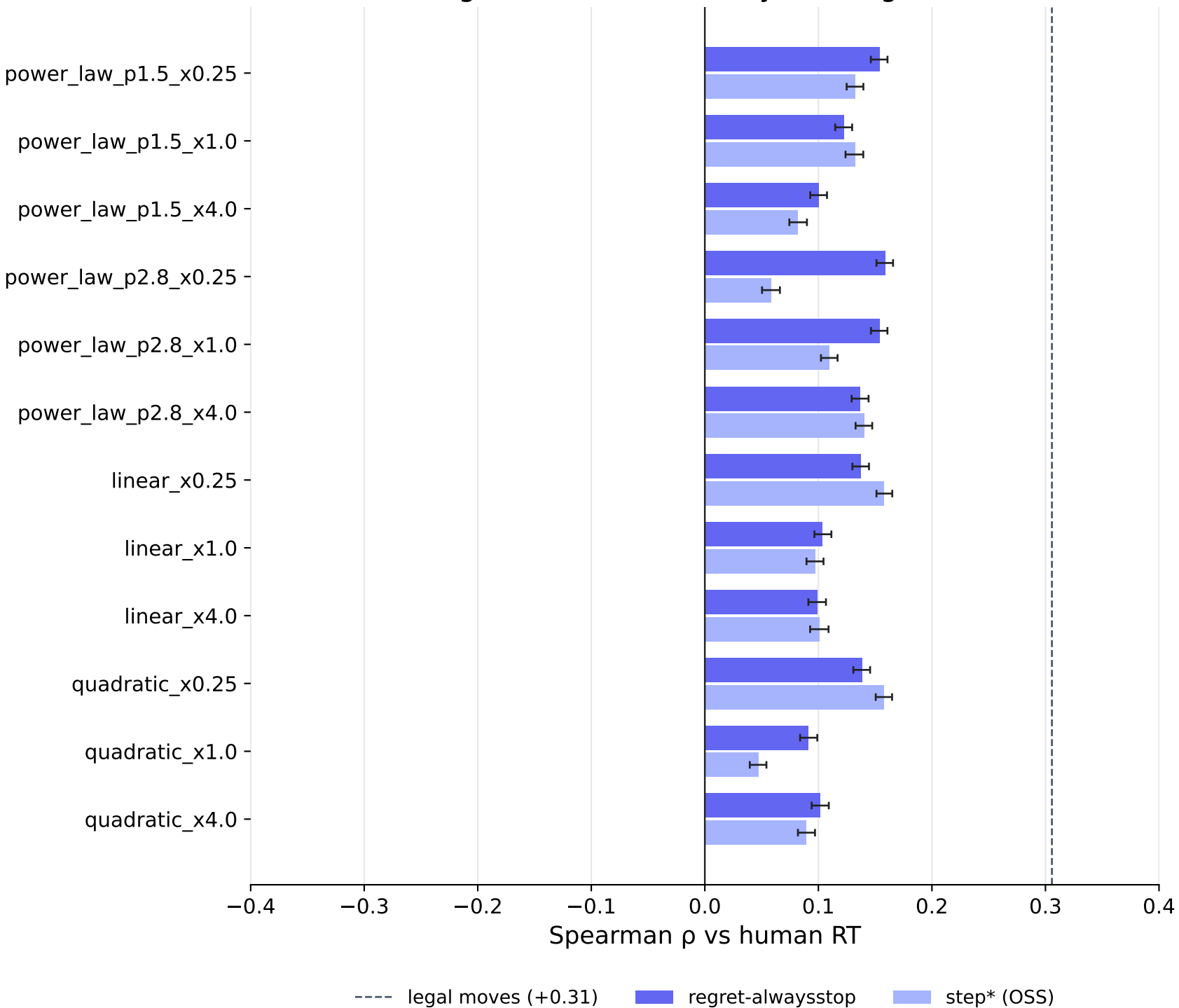
Normative signals vs human RT, by cost regime (n=64,751)
