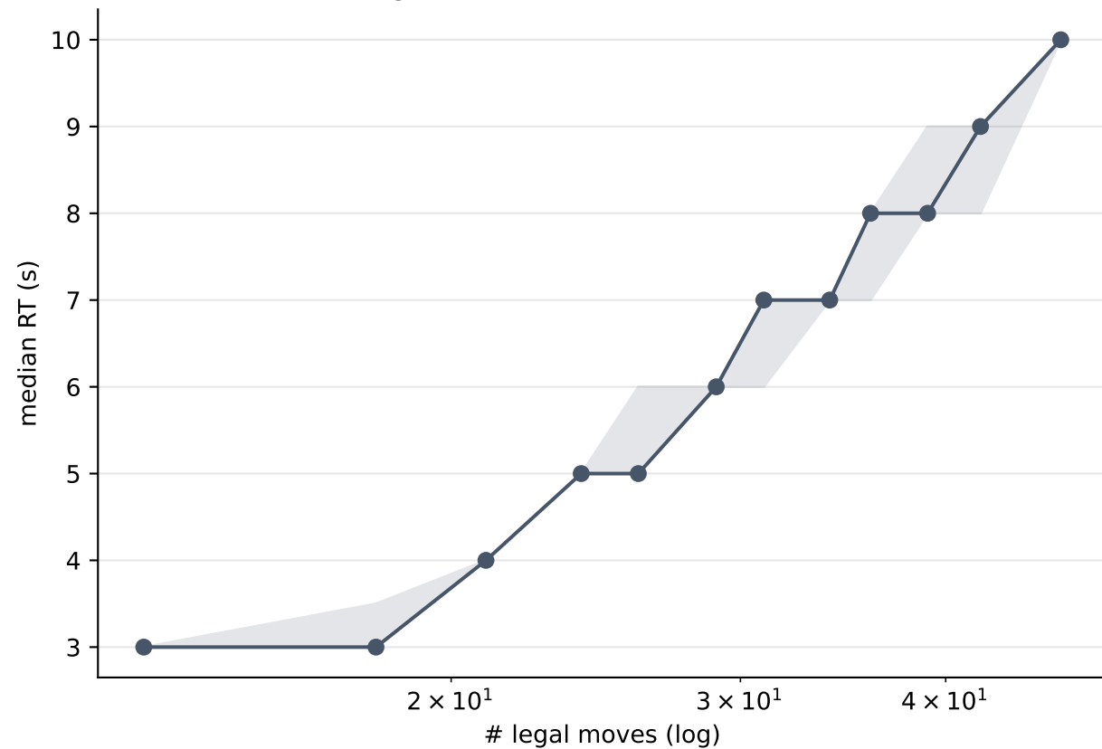
RT vs legal moves — concave? log-fit R^2=0.085 vs linear R^2=0.095
