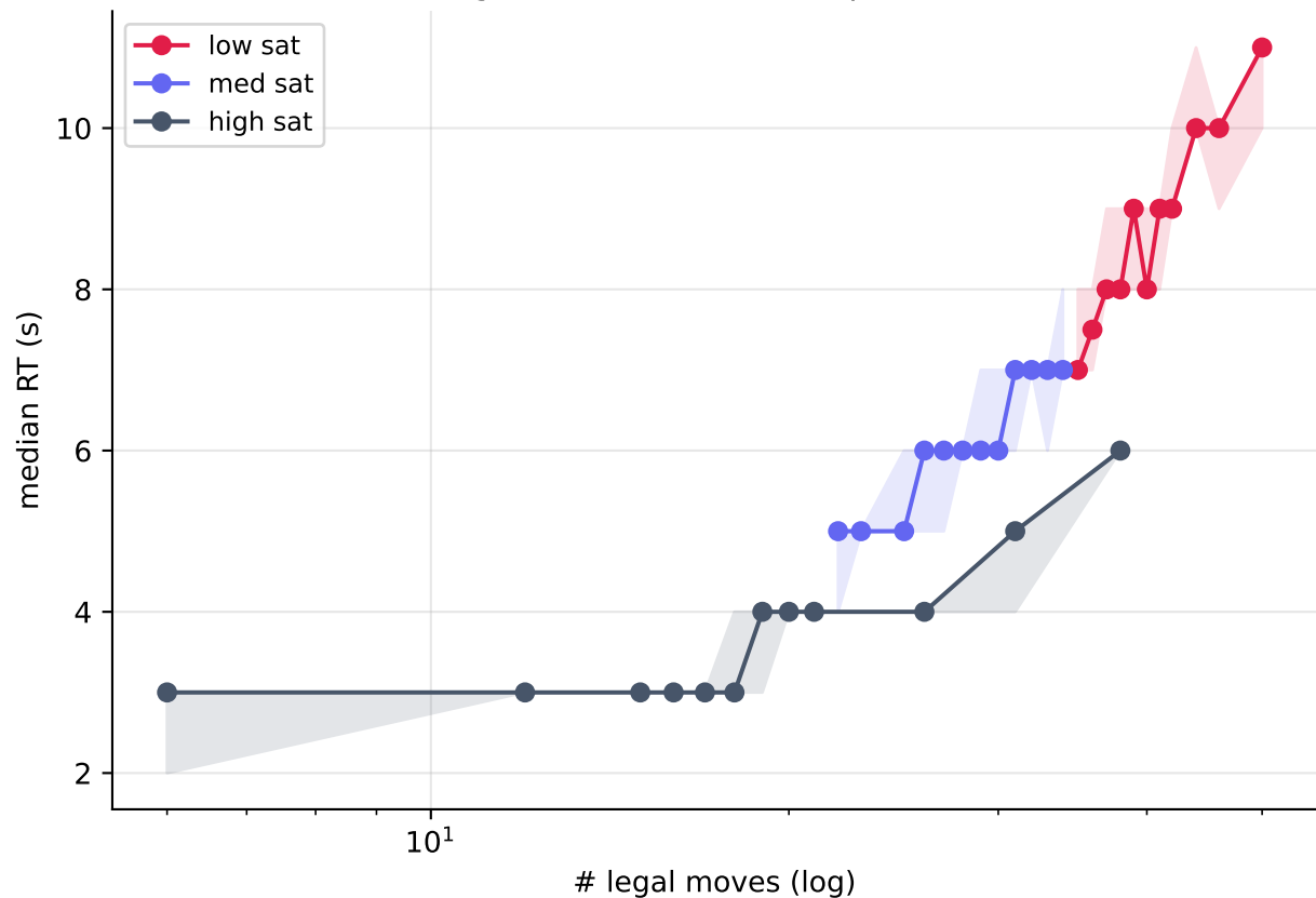
Plateau shift by satisfaction (high satisfaction \Rightarrow lower plateau?)
