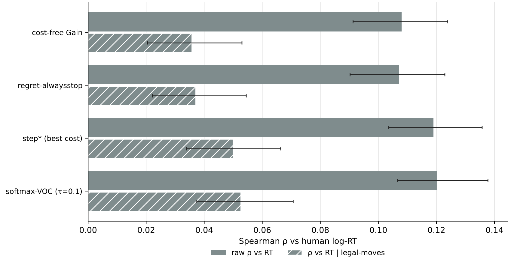
Value-of-computation signals are proxies for legal-moves (n=13,051)
