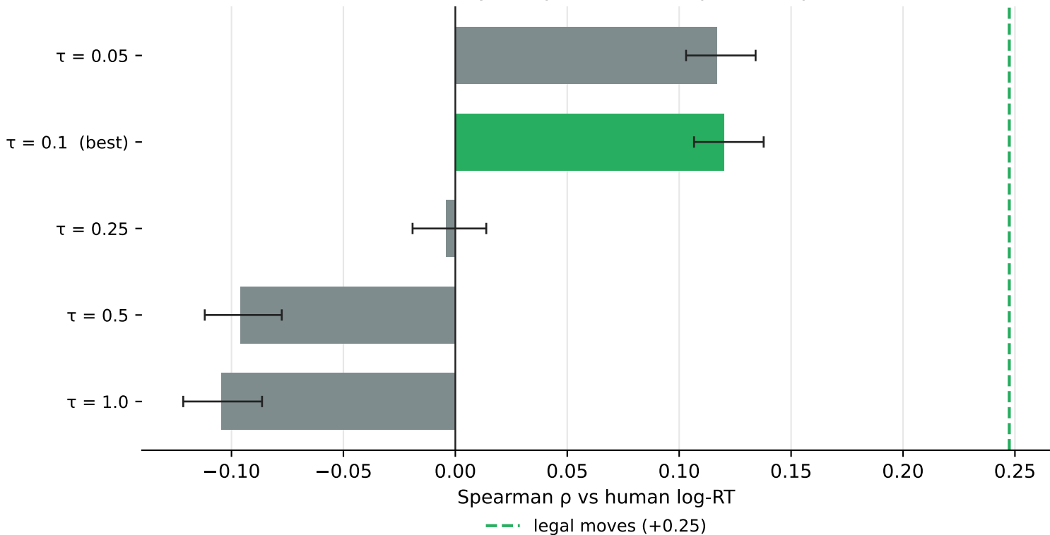
Softmax-VOC vs human RT, by temperature (deep-tree supervisor) (n=13,051)
