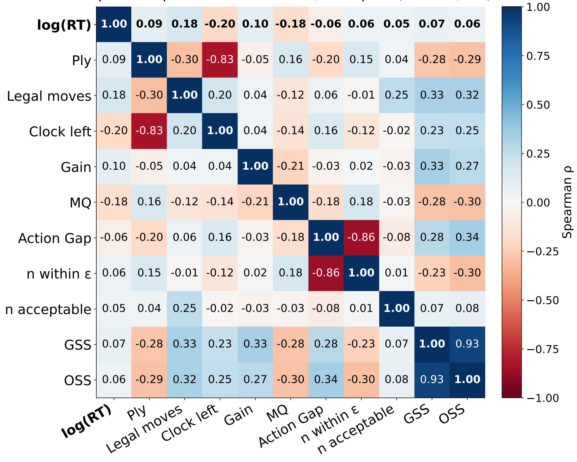
Spearman \rho — SF-1 BeFS metrics, unit=pwin (n = 102,075)
