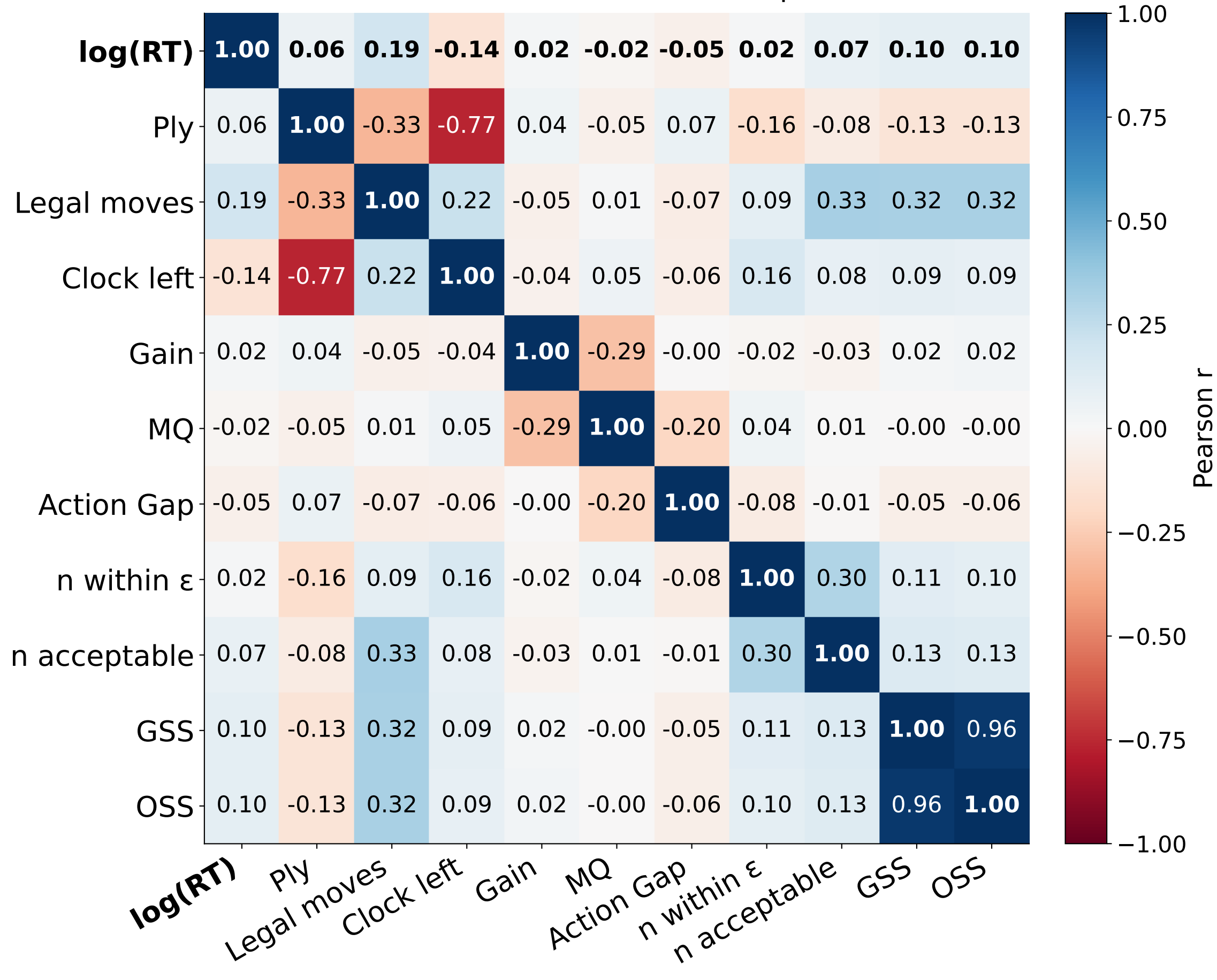
Pearson r — SF-1 BeFS metrics, unit=cp (n = 104,922)
