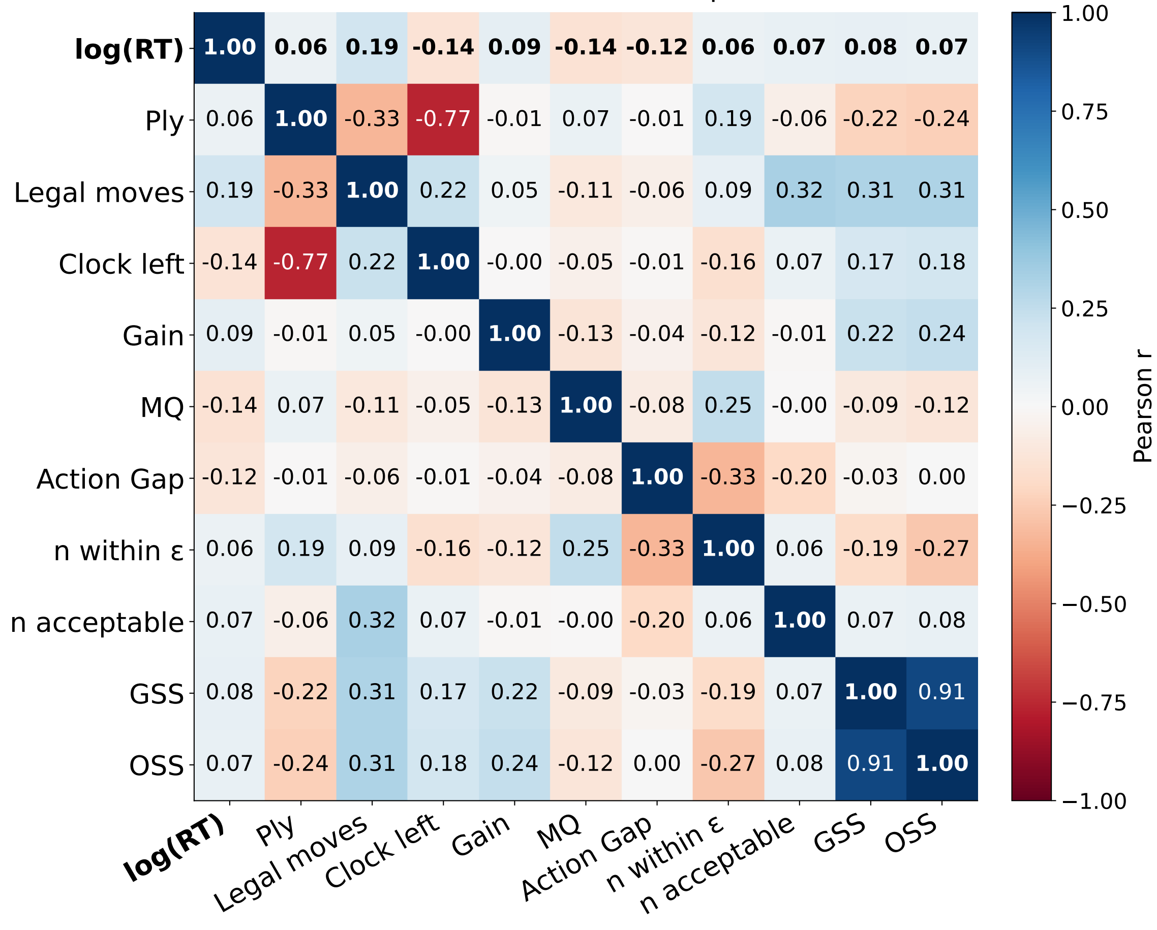
Pearson r — SF-1 BeFS metrics, unit=pwin (n = 104,922)
