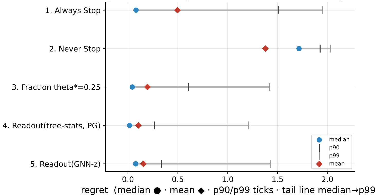
Regret distribution by model (mean \gg median \Rightarrow heavy tail)
