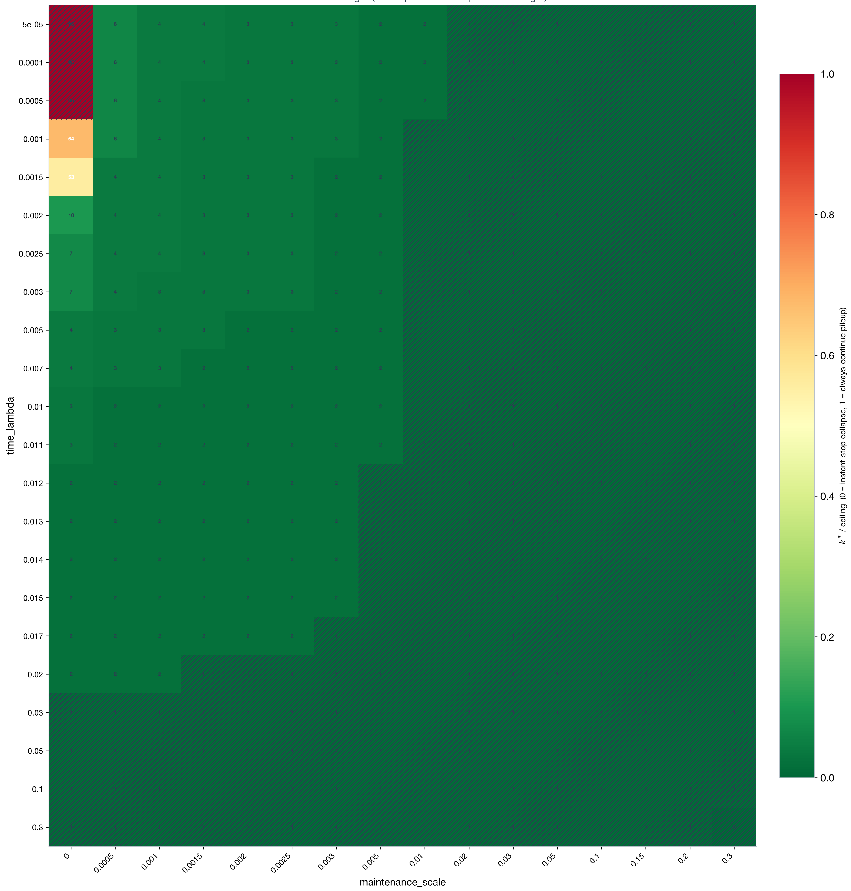
REGIME sweep: SingleHalt*'s own k^* (cell text) across cost regimes hatched = NOT meaningful ( k^* collapsed to \leq 1 or pinned at ceiling-1)
