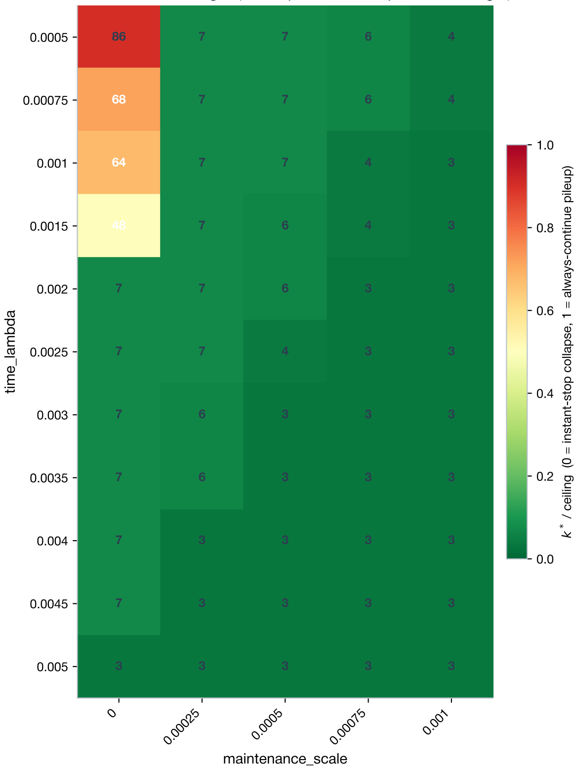
REGIME sweep: SingleHalt*'s own k^* (cell text) across cost regimes hatched = NOT meaningful ( k^* collapsed to \leq 1 or pinned at ceiling-1)
