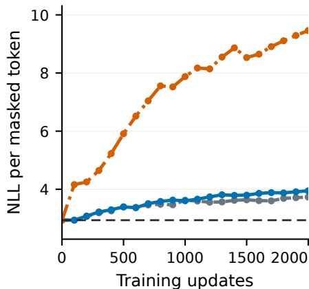
Held-out examples
