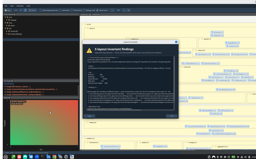
Figure 1: R2 checker report: packages in a filtered package-SCC occupy different levels. The checker reports findings as algorithm-bug candidates with a reproducer block, which makes the visual failure traceable to concrete level-pipeline consistency conditions.
