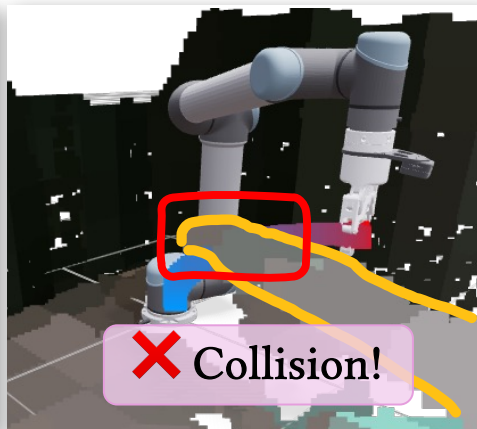
Baseline, t=0
