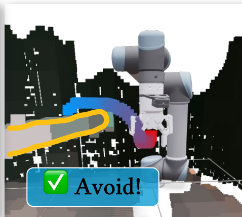
Ours, t=0
