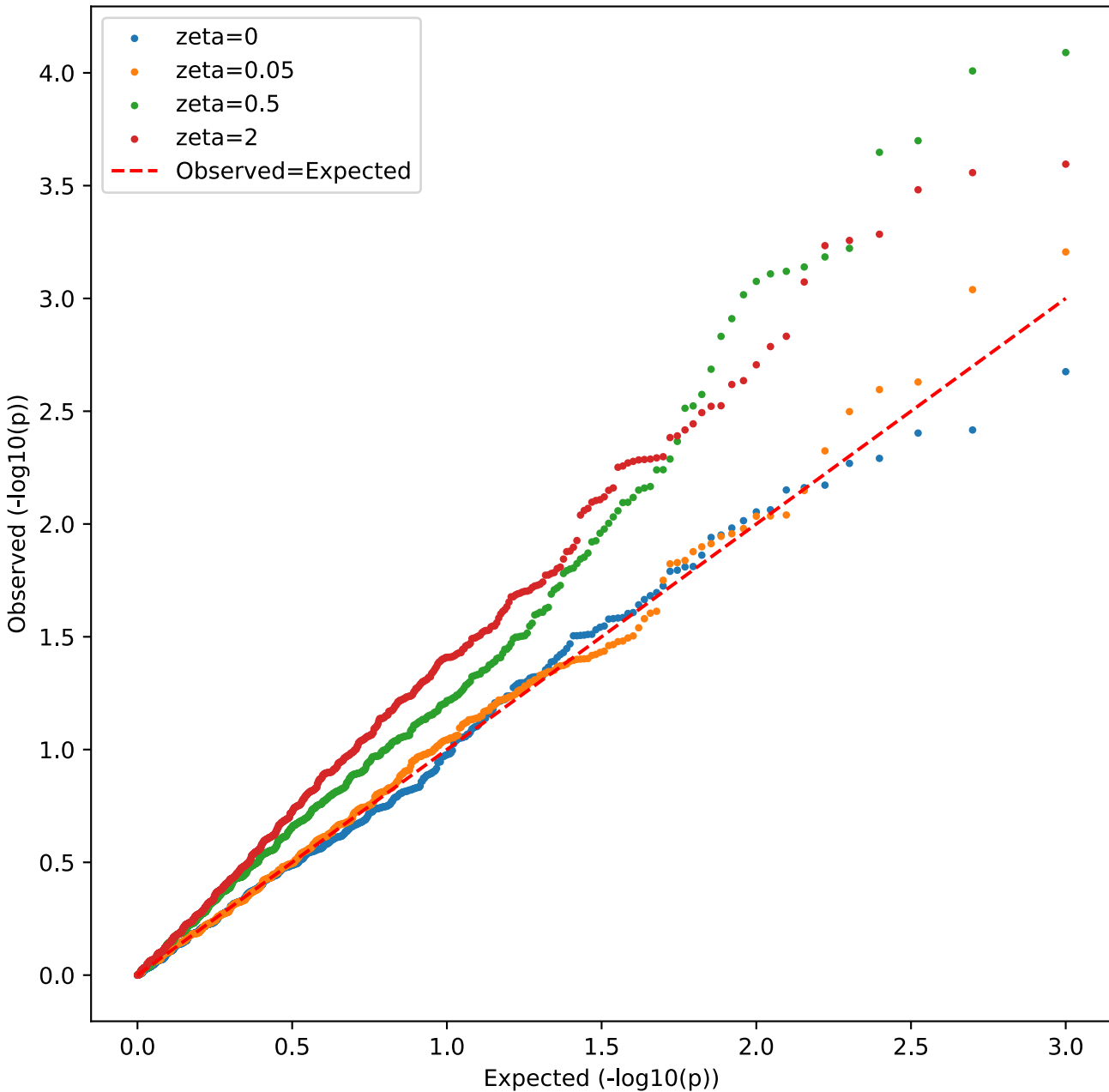
QQ-plot (Sensitivity analysis)
