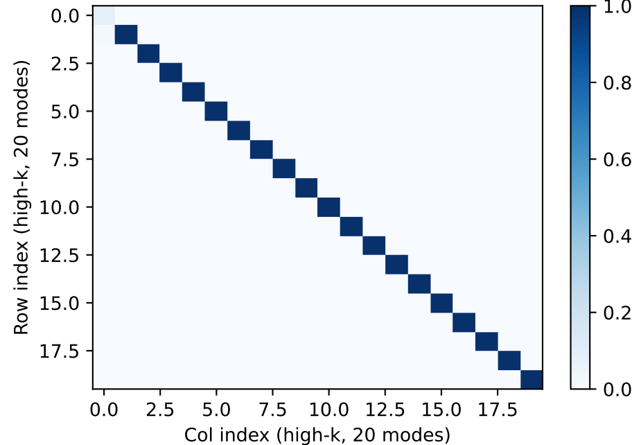
|M[\text{high-k block}]| — fwd ordering (should be \approx I , \|\cdot-I\|_F=0.907 )
