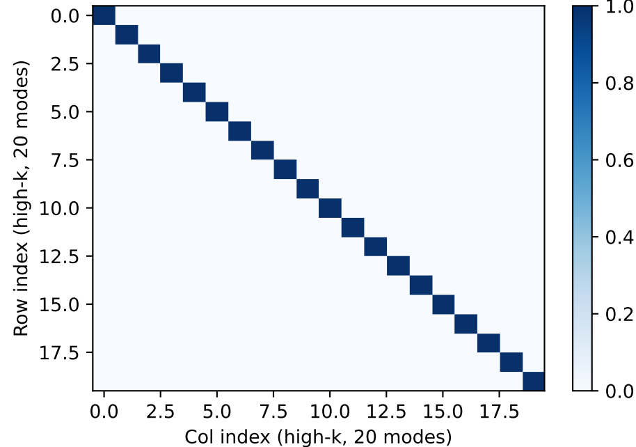
|M[\text{high-k block}]| — rev ordering (should be \approx I , \|\cdot-I\|_F=0.000 )
