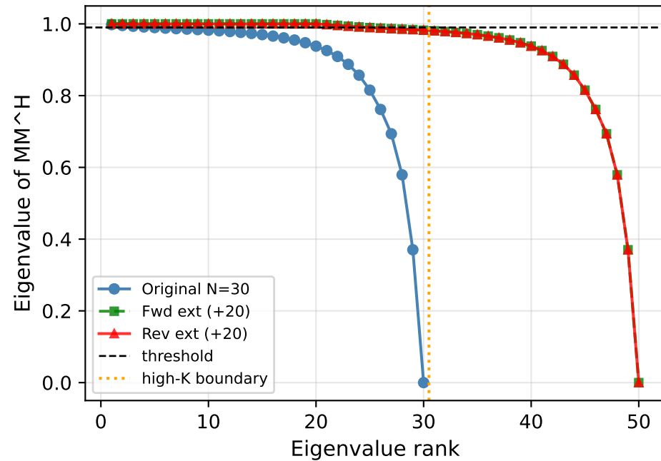
Eigenvalue spectra (all three cases)
