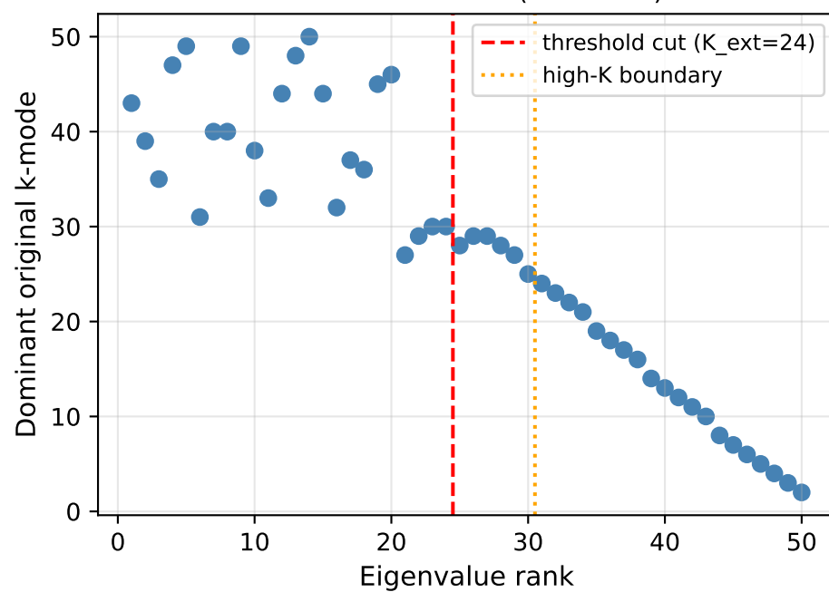
Dominant k-mode (extended)
