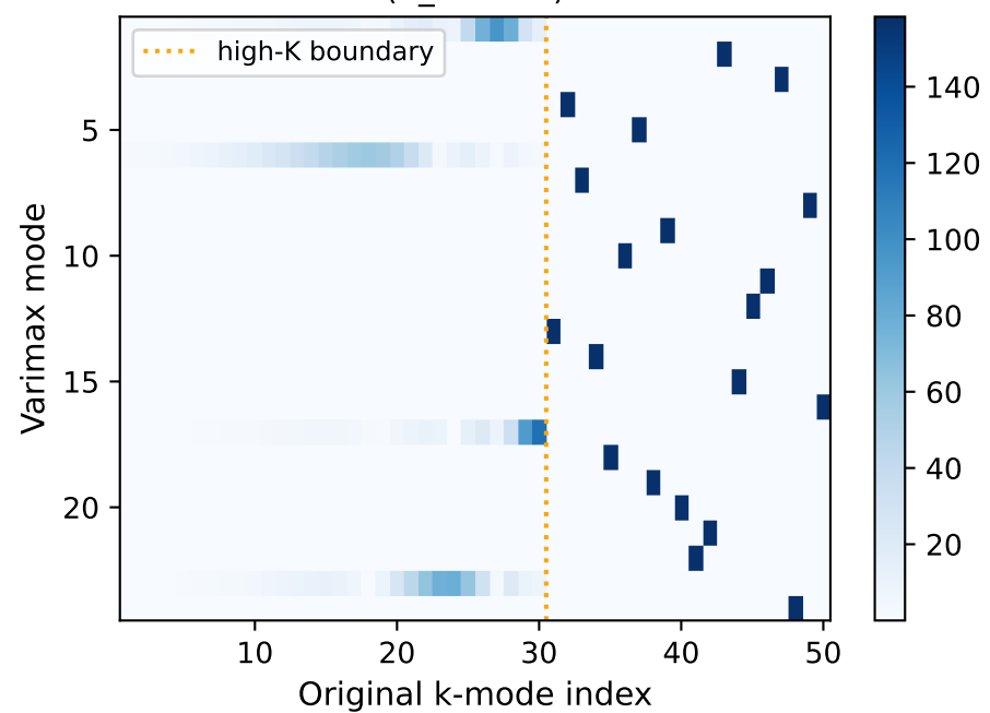
Sparse coefficients (extended) ( K_{\text{ext}}=24 )
