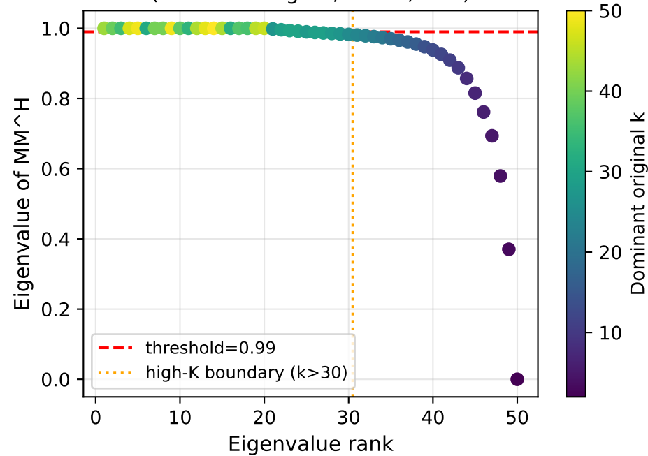
Extended eigenvalue spectrum ( N=30+20 high-K, \kappa=1.5 , T=\pi )
