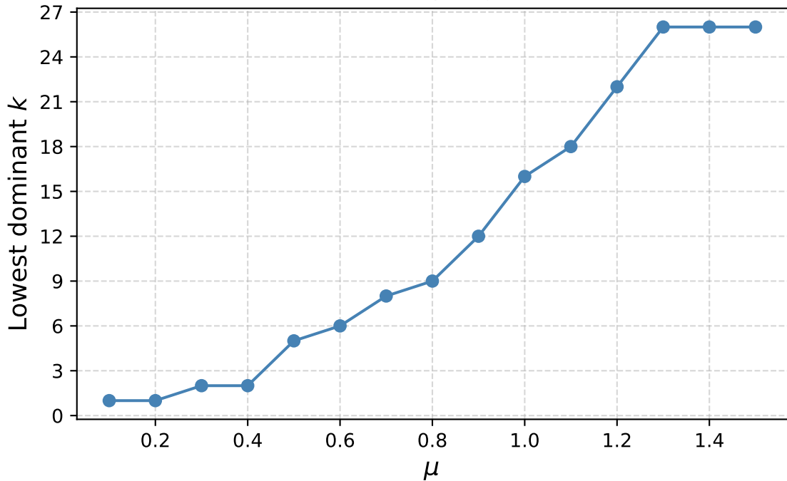
Lowest dominant k vs \mu (eigenvalue > 0.99 )
