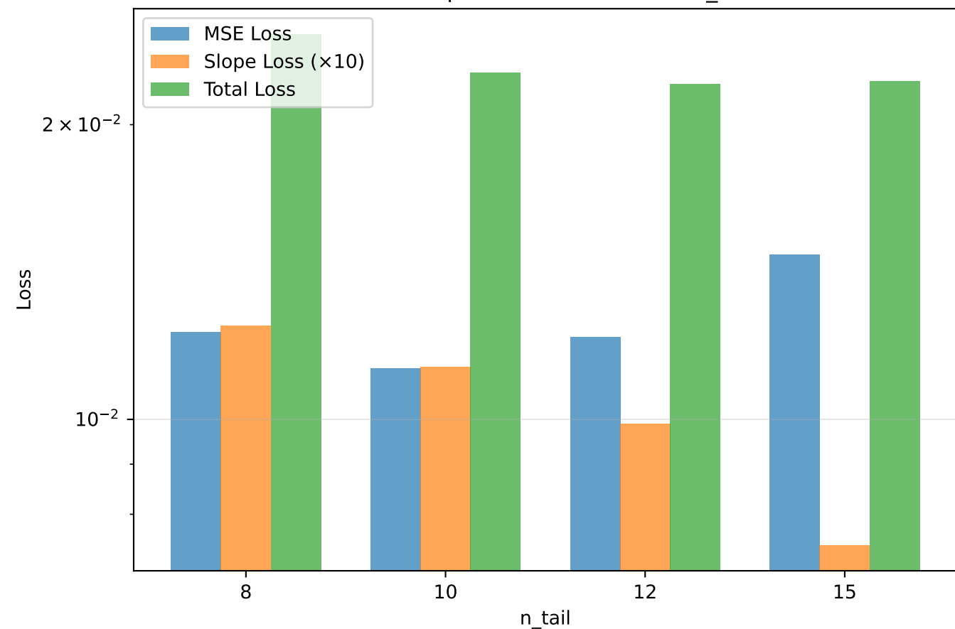
Loss Components for Different n_tail
