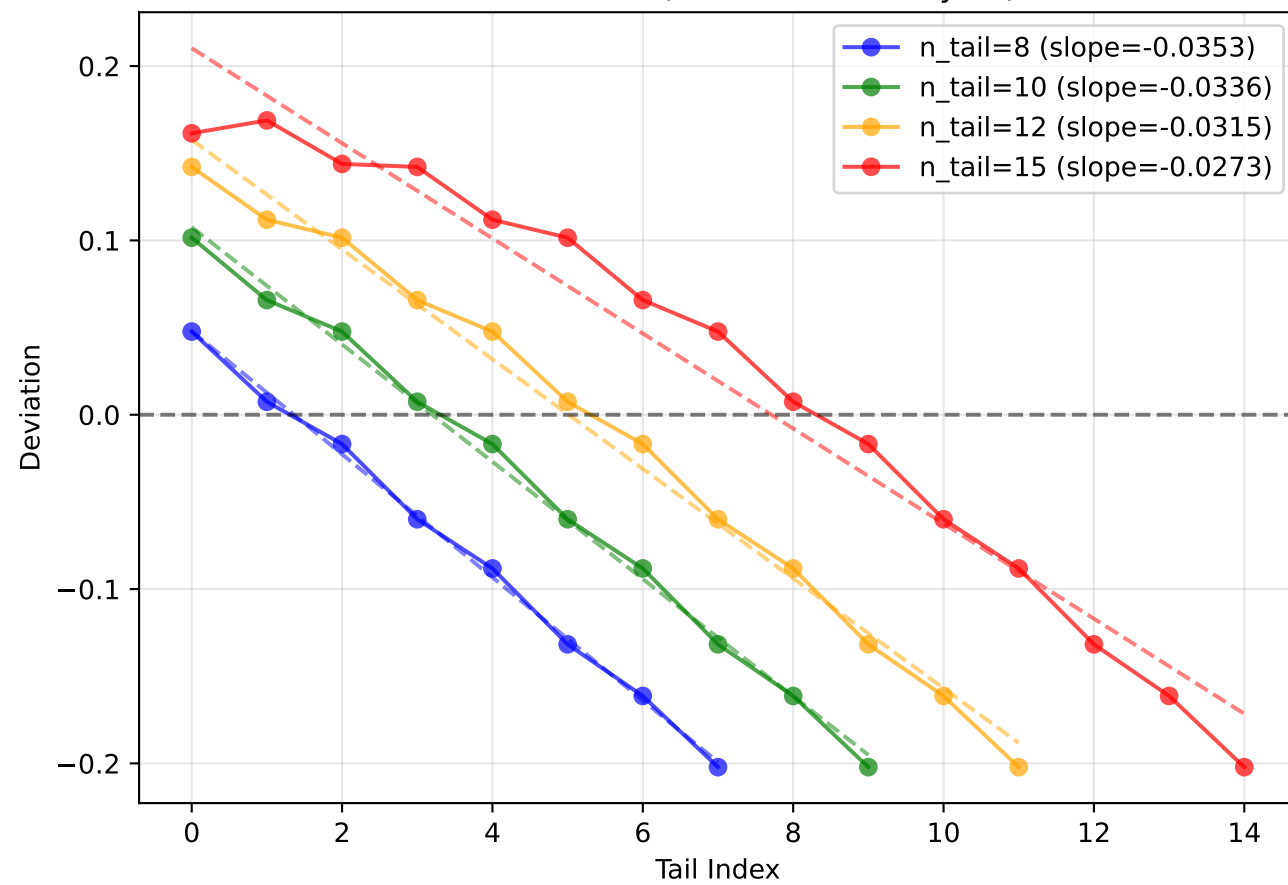
Tail Deviations (Goal: flat line at y=0)
