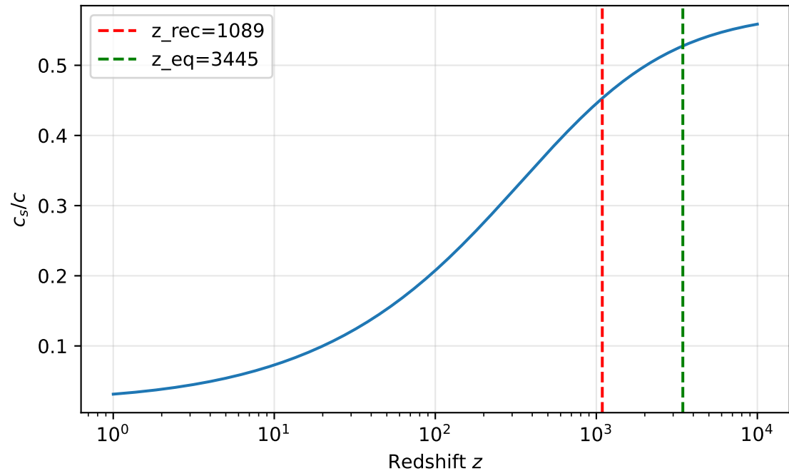
Sound speed c_s(z)
