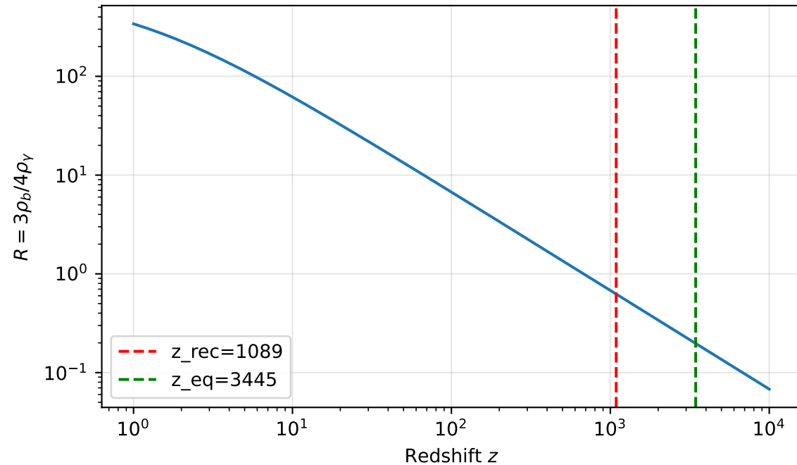
Baryon-to-photon ratio R(z)
