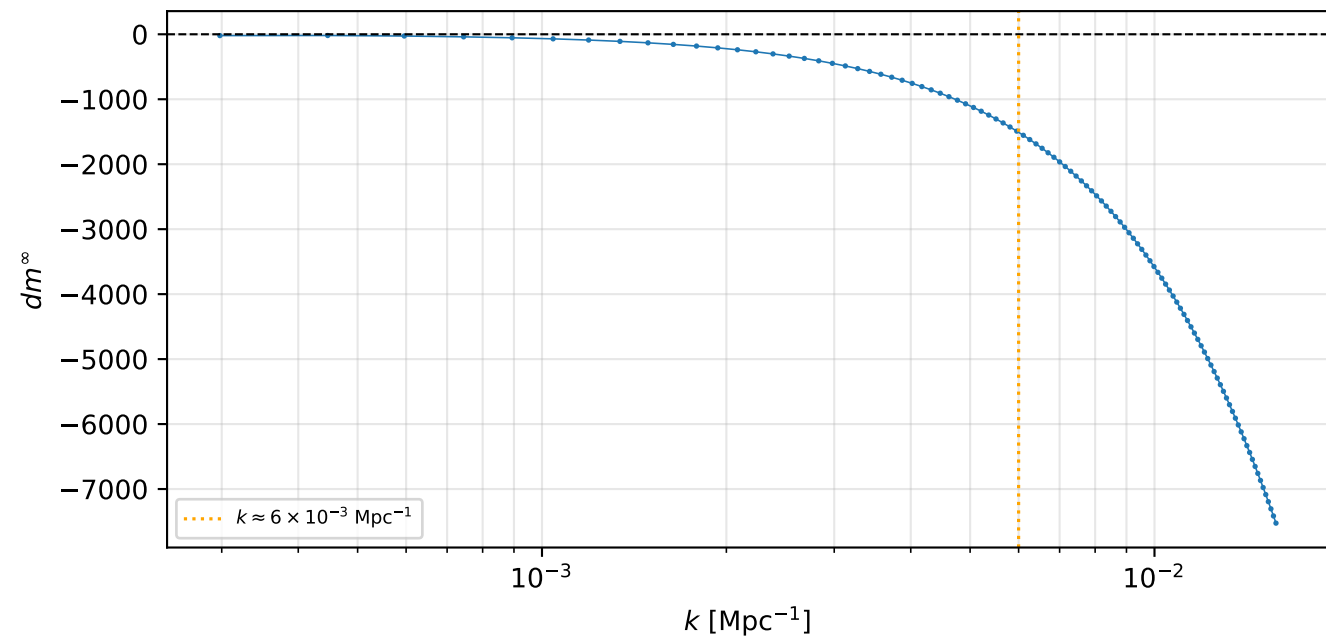
dm^\infty at FCB (integerK)
