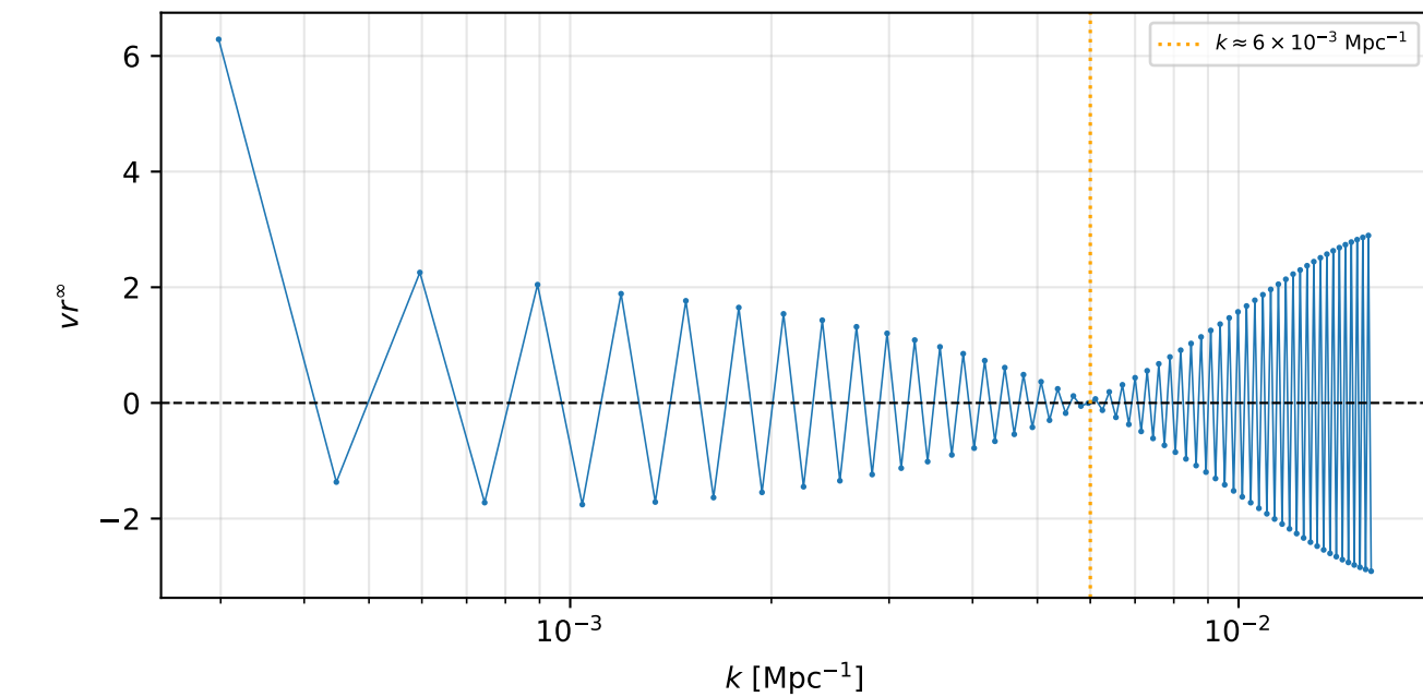
vr^\infty at FCB (integerK)
