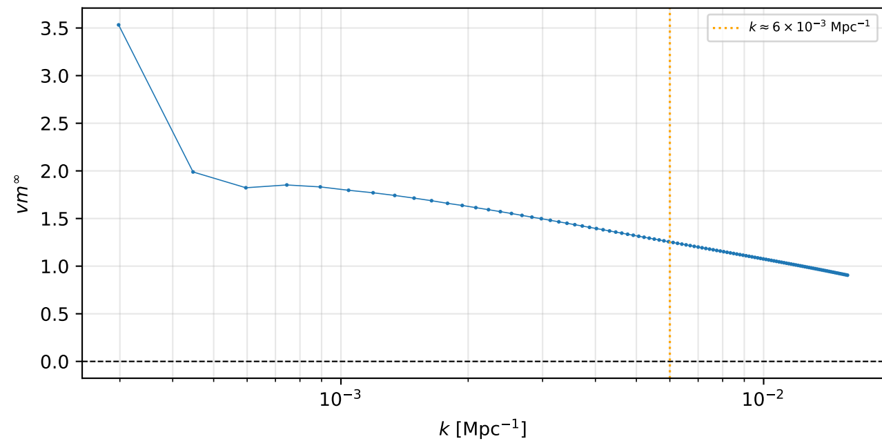
vm^\infty at FCB (integerK)
