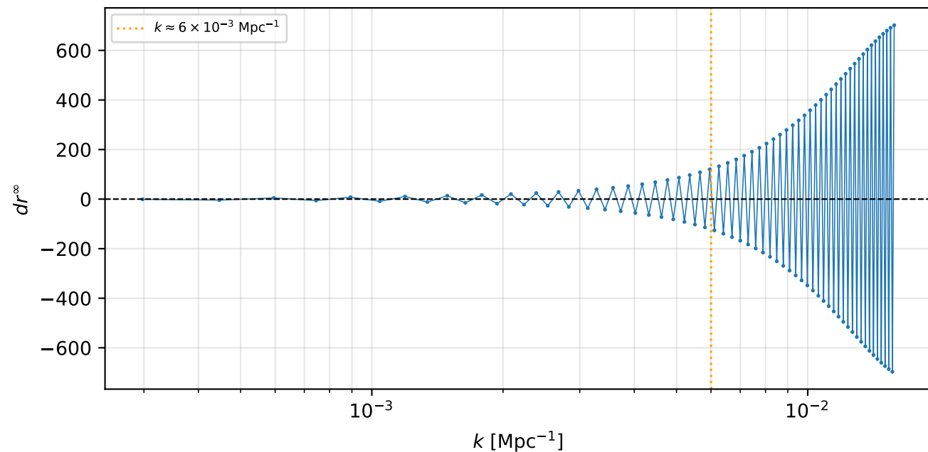
dr^\infty at FCB (integerK)
