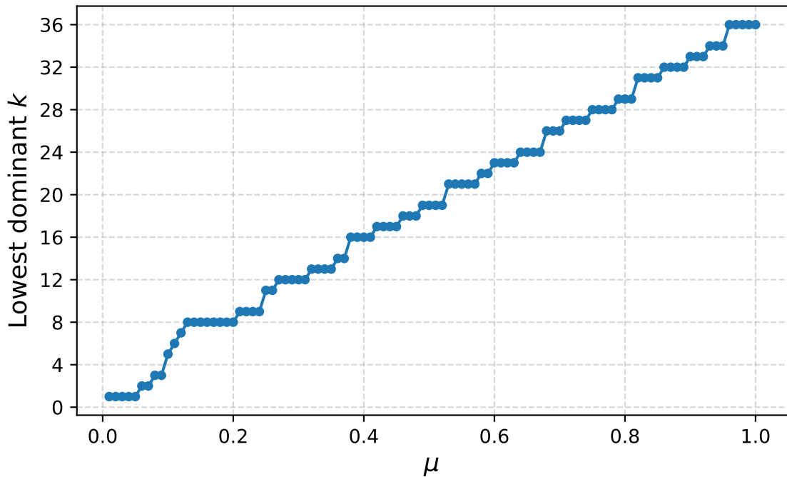
Lowest dominant k vs \mu
