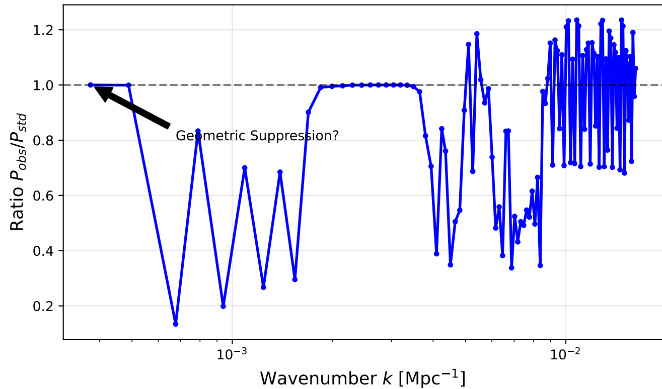
Ratio of Double-BC PPS to Standard Power Law
