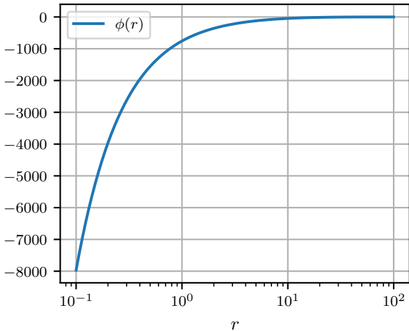
\phi(r) with NFW profile
