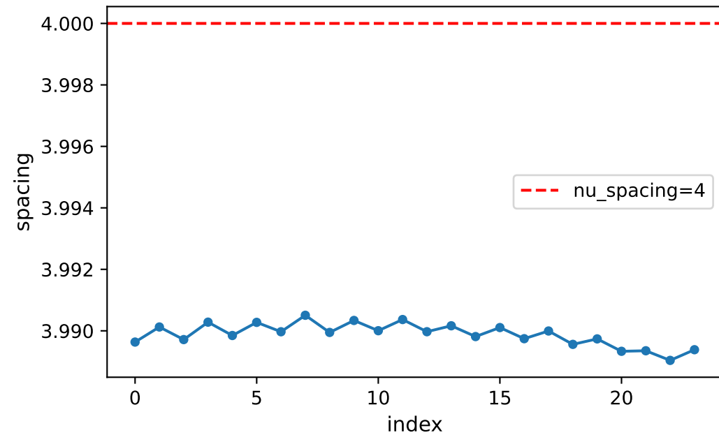
Best trial: consecutive spacings
