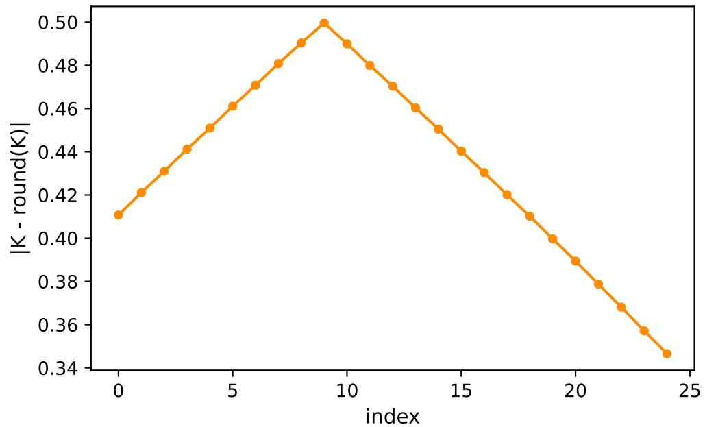
Best trial: deviation of K from nearest integer
