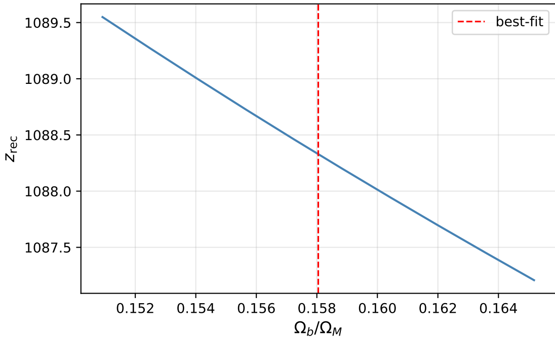
z_{\text{rec}} vs \Omega_b/\Omega_M (other params fixed at best-fit)
