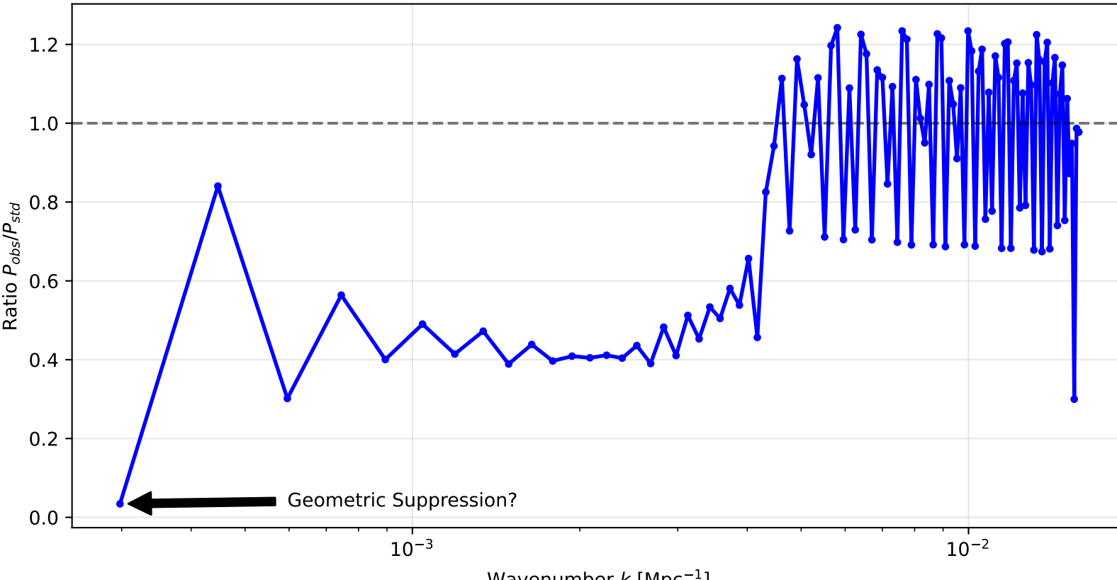
Ratio of Double-BC PPS to Standard Power Law
