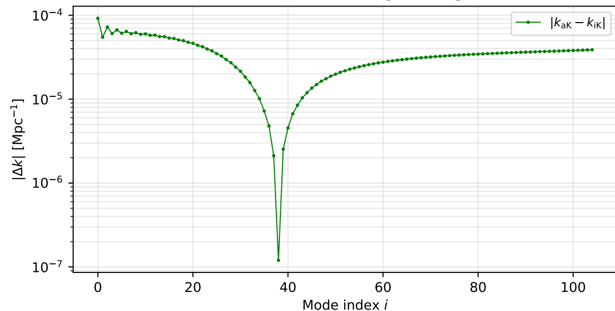
(b) Absolute \Delta k (converges at high k )
