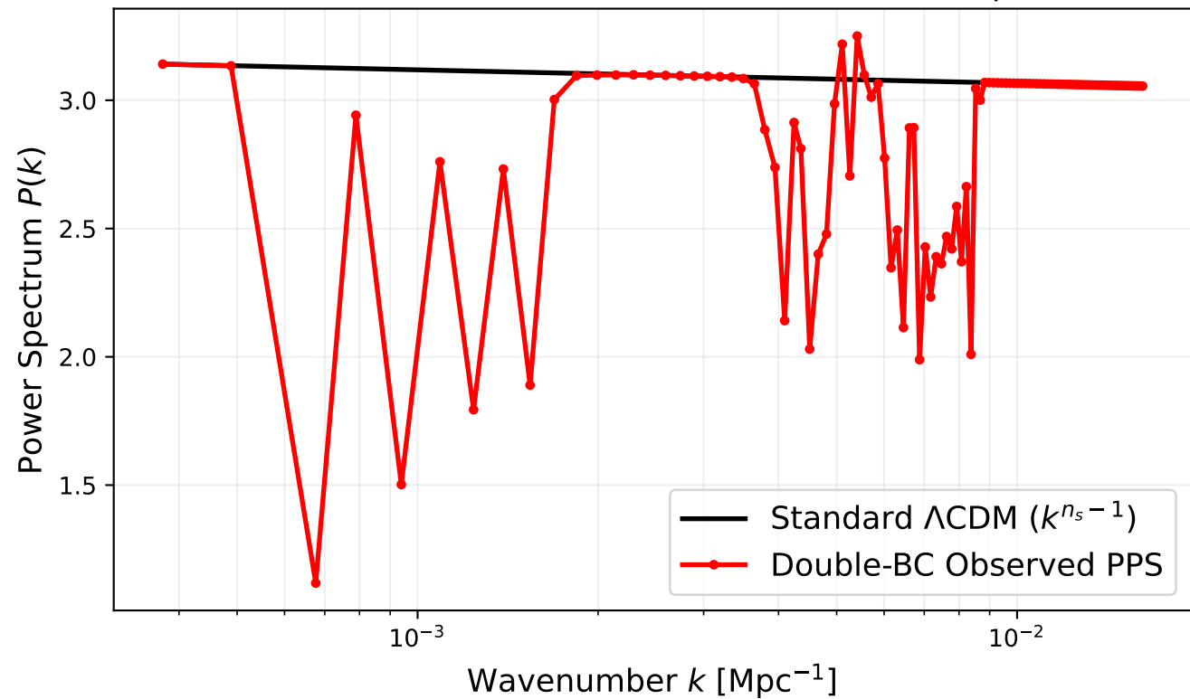
Prediction: Geometric Modulation of the Power Spectrum
