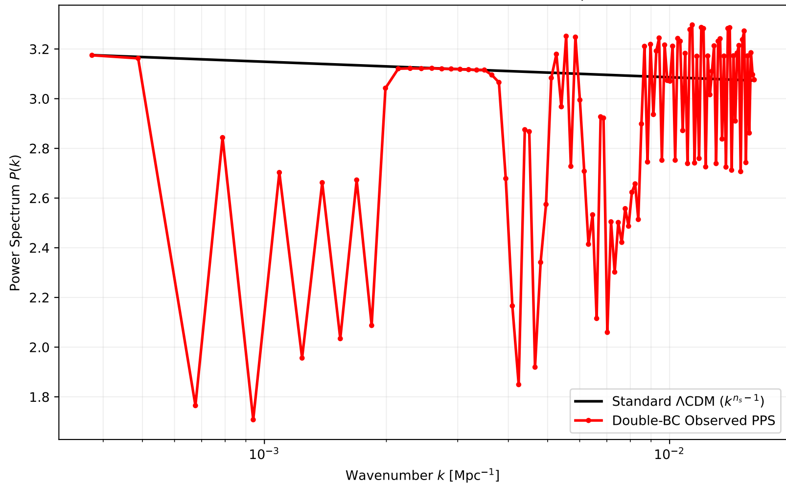
Prediction: Geometric Modulation of the Power Spectrum
