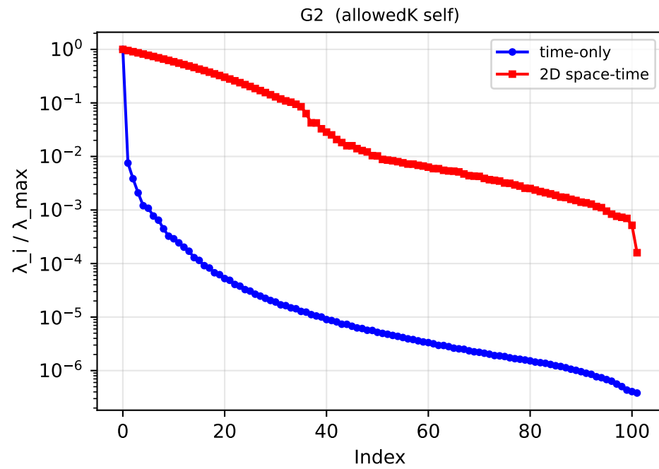
Gram eigenvalue spectra: time-only vs 2D space-time
