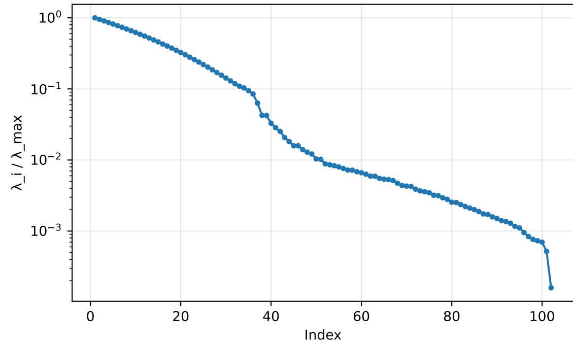
Gram eigenvalue spectrum: G2 (allowedK)
