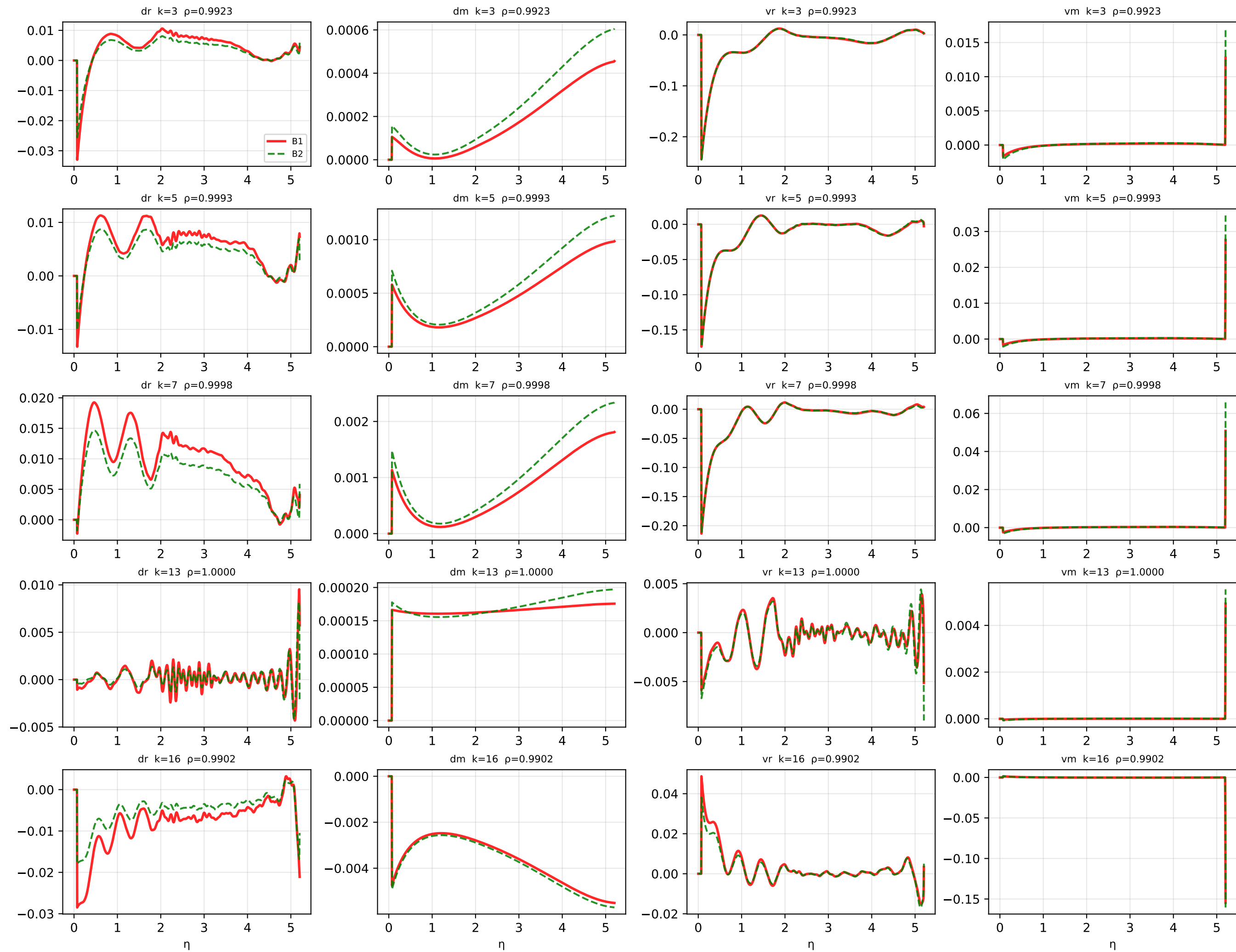
CCA sparse modes: time-series (Basis 1 red vs Basis 2 green, Frobenius-normalised)
