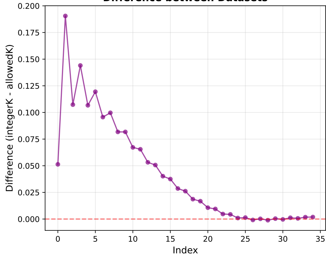
Difference between Datasets
