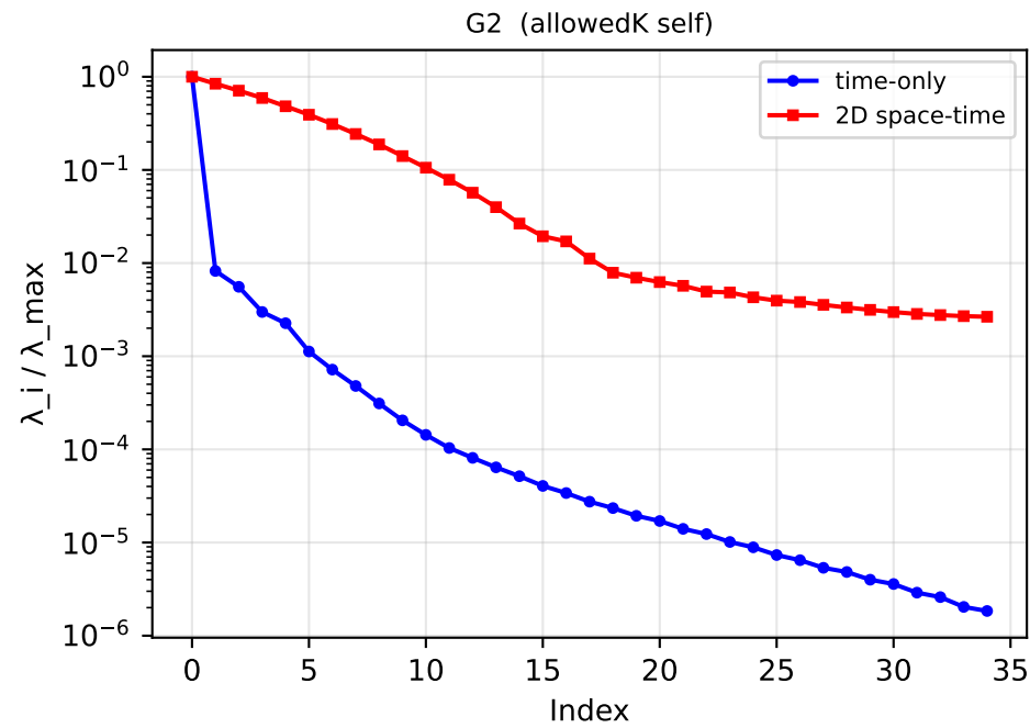
Gram eigenvalue spectra: time-only vs 2D space-time
