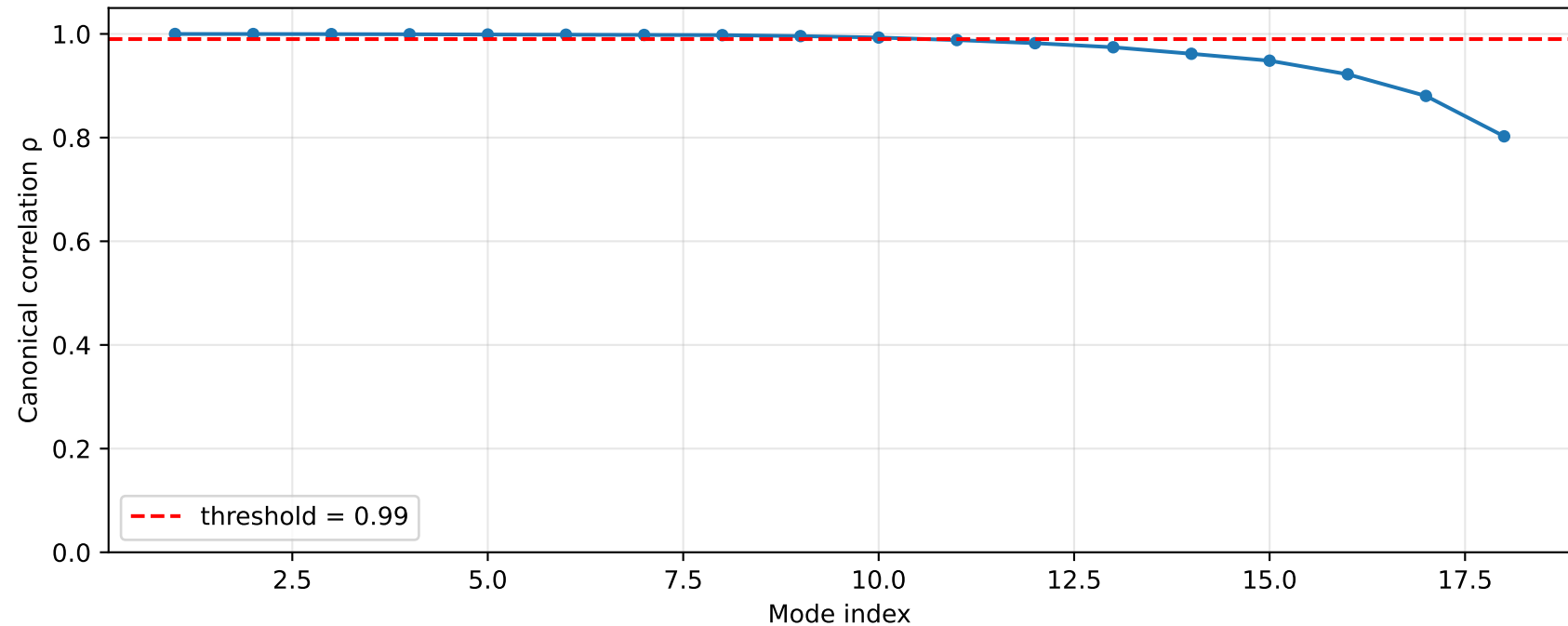
CCA: canonical correlations between Basis 1 and Basis 2
