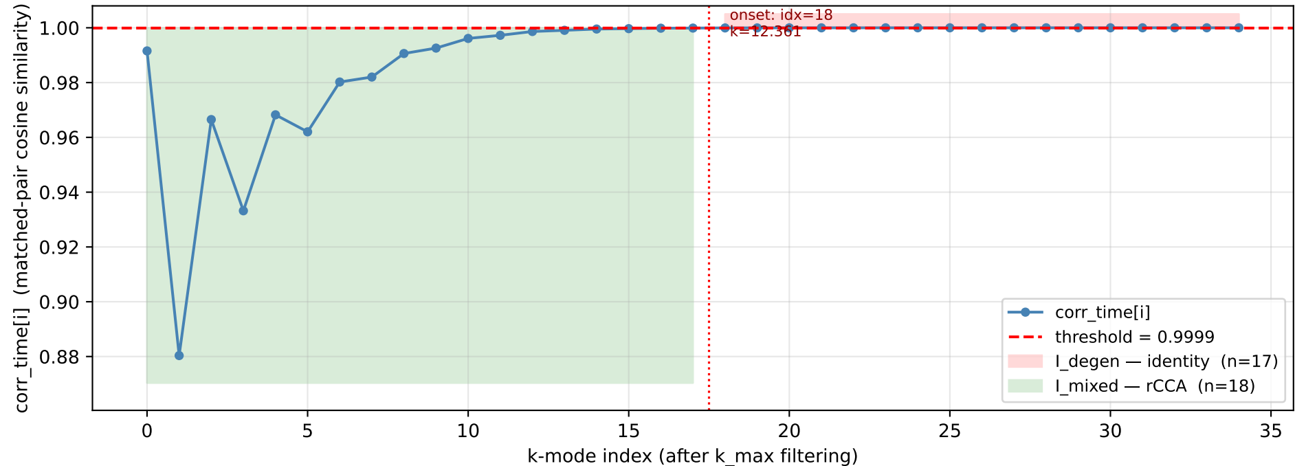
Partition: I_degen (identity) vs I_mixed (rCCA)
