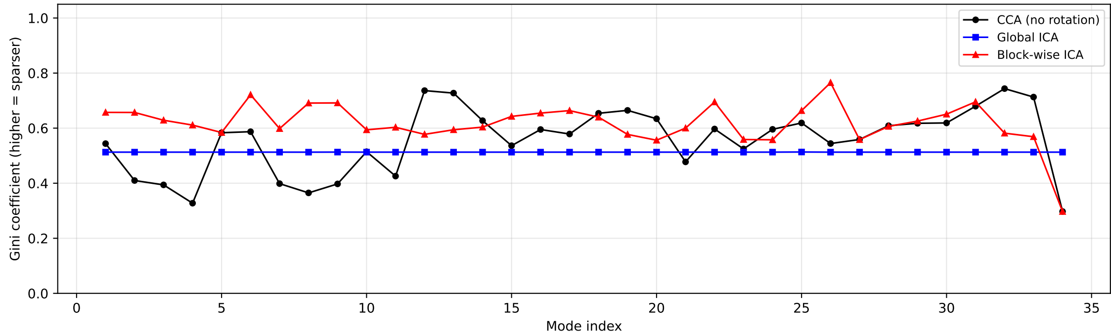
Sparsity per mode: original CCA vs ICA variants
