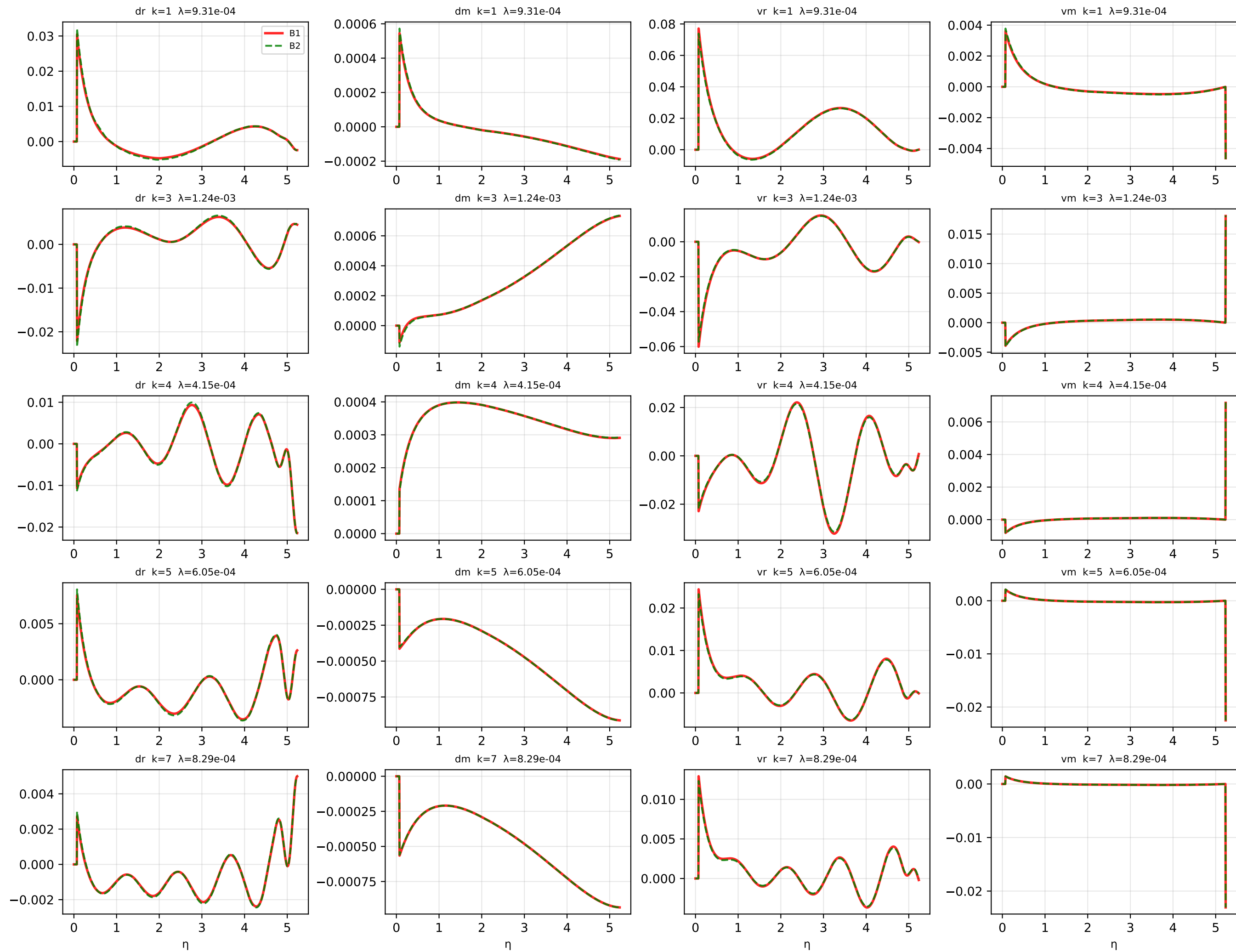
Match-solution sparse modes: time-series (Basis 1 red vs Basis 2 green, Frobenius-normalised)
