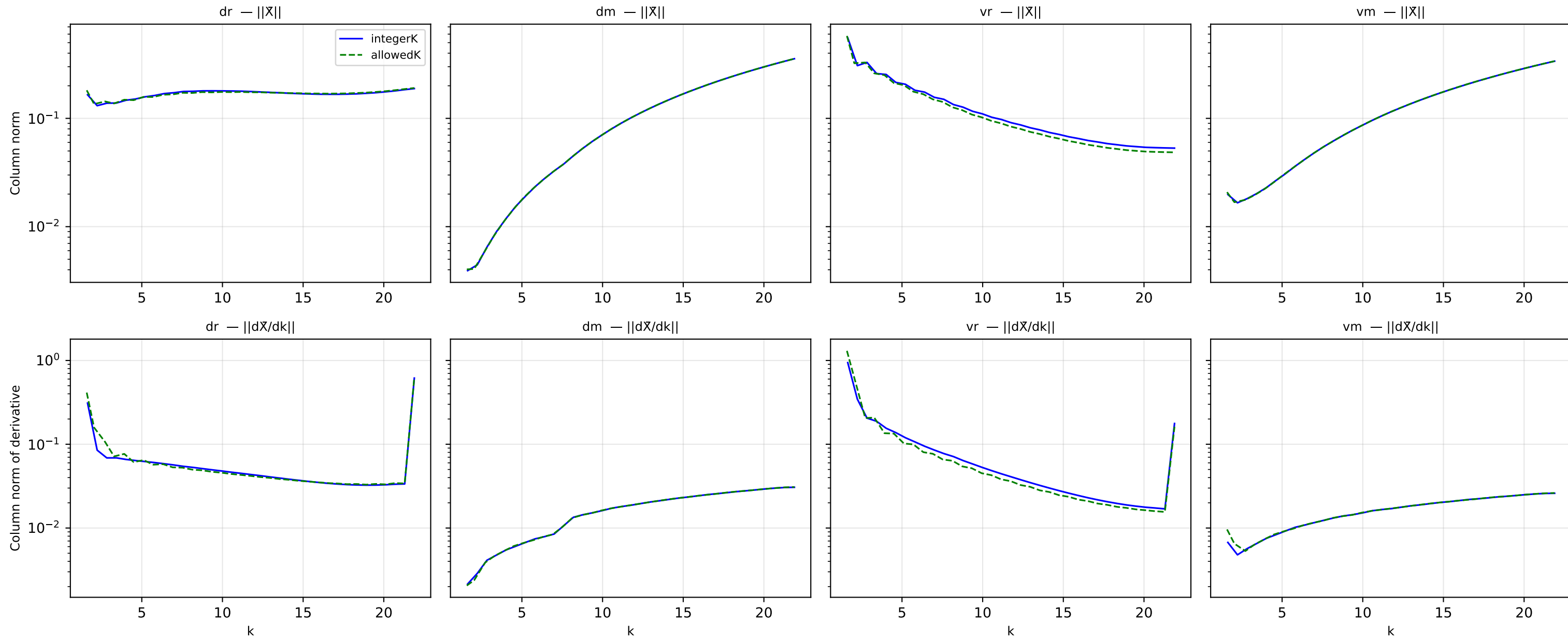
Column norms: ||\tilde{X}(:,i)|| and ||d\tilde{X}/dk(:,i)|| vs k
