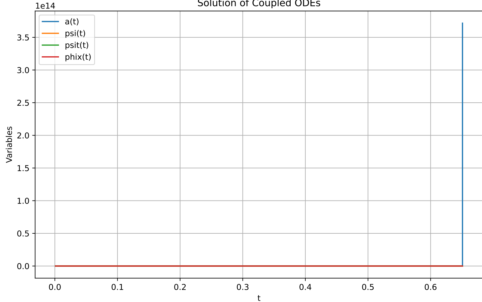
Solution of Coupled ODEs
