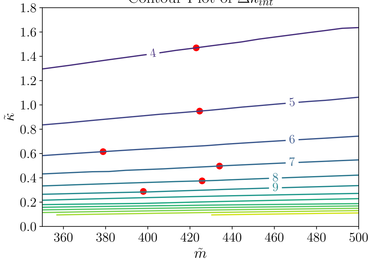
Contour Plot of \Delta k_{int}
