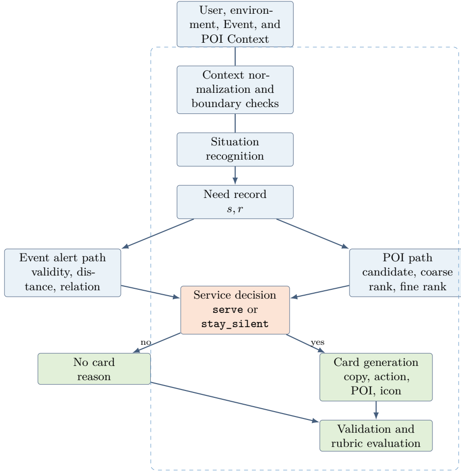
Figure 1: The Context-to-Card architecture. Light nodes are transformations, orange nodes are service gates, green nodes are externally visible or evaluable outputs, and the dashed boundary marks the shared method. The need record is the explicit interface between context interpretation and service execution.
