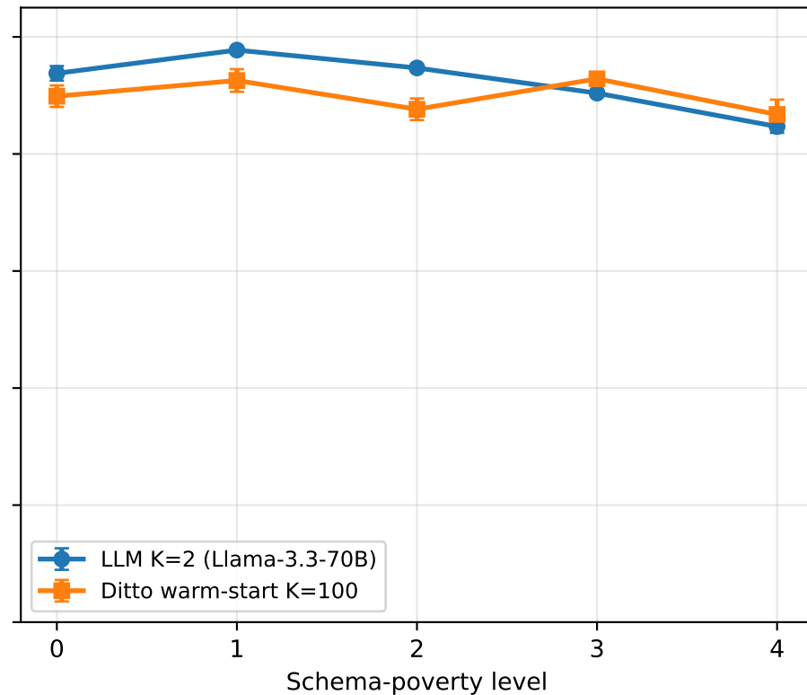
DBLP-ACM (citation)
