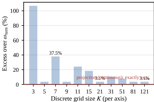
(a) Compliance-turn granularity (not monotone in K )
