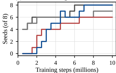
(e) Seeds reaching the 50% criterion
