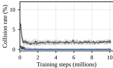
(c) Collision rate (training)
