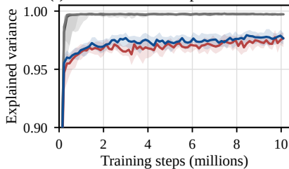
(f) Value-function explained variance
