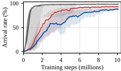
(b) Arrival rate (training)
