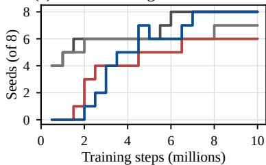
(e) Seeds reaching the 50% criterion
