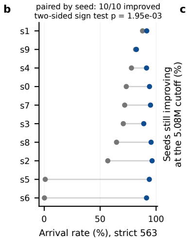
Fig. 1 | Sample efficiency under an identical training budget. a, Learning curves (thin: individual seeds; thick: median). b, Same-seed pairing on the official test set. c, Fraction of non-collapsed seeds whose last three segments still improve by more than two standard errors — the old recipe has not converged at the cutoff, so the comparison is a sample-efficiency claim, not a converged-performance claim. 5.08M-step budget · last checkpoint · official test set (strict 563) · single machine, single pass
