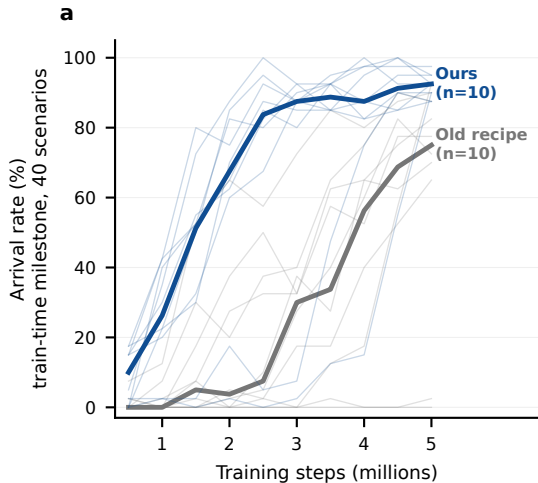
Fig. 1 | Sample efficiency under an identical training budget. a, Learning curves (thin: individual seeds; thick: median). b, Same-seed pairing on the official test set. c, Fraction of non-collapsed seeds whose last three segments still improve by more than two standard errors — the old recipe has not converged at the cutoff, so the comparison is a sample-efficiency claim, not a converged-performance claim. 5.08M-step budget · last checkpoint · official test set (strict 563) · single machine, single pass
