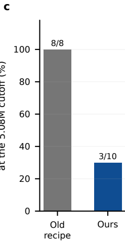
Fig. 1 | Sample efficiency under an identical training budget. a, Learning curves (thin: individual seeds; thick: median). b, Same-seed pairing on the official test set. c, Fraction of non-collapsed seeds whose last three segments still improve by more than two standard errors — the old recipe has not converged at the cutoff, so the comparison is a sample-efficiency claim, not a converged-performance claim. 5.08M-step budget · last checkpoint · official test set (strict 563) · single machine, single pass
