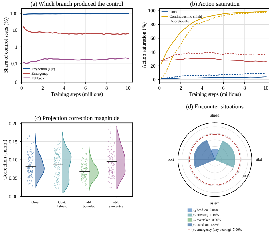
Figure 4 Behavior of the shield during training. In panel (d) the angle is the sector in which the convention defines each situation, not the measured bearing distribution of target vessels, and the radius is logarithmic. This figure is collected during training rather than at evaluation.
